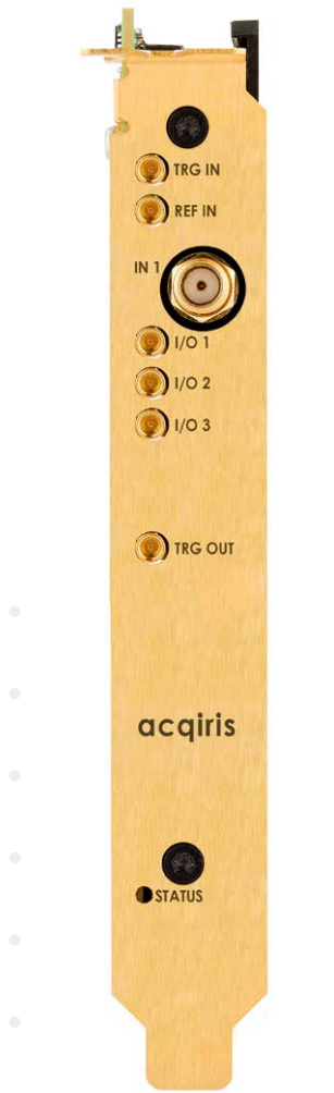
Figure 3. SA230P front panel, with analog inputs and multiple programmable I/O signals.
