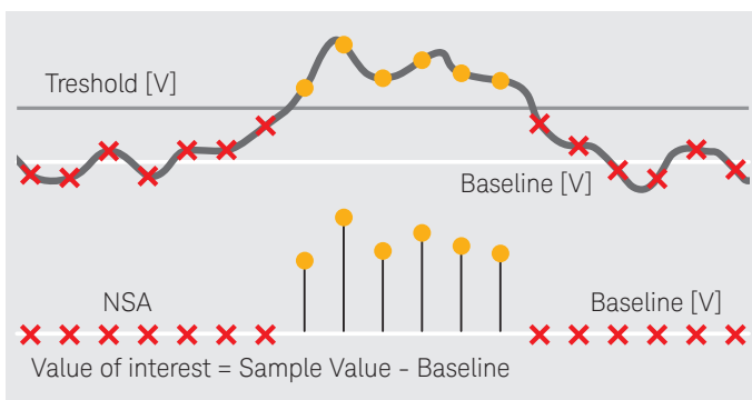
Figure 3. Signal detection using noise suppressed accumulation
