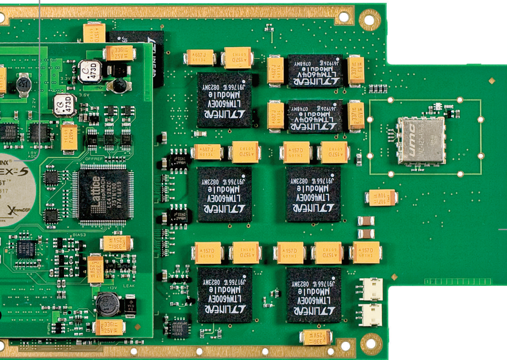
Figure 1. U1084A high-speed digitizer card.
